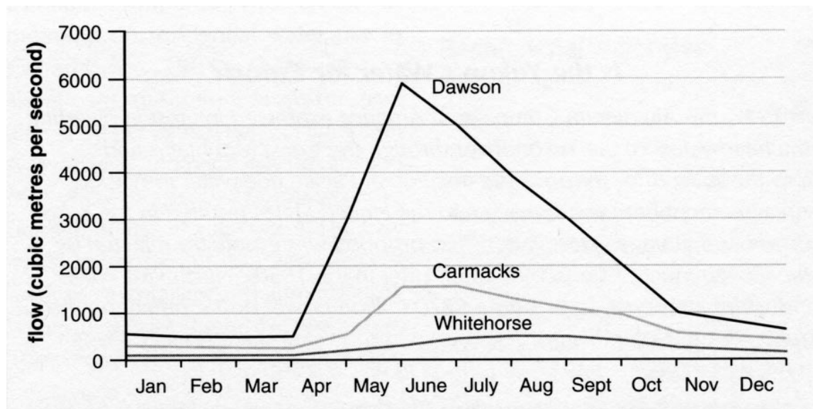
Figure 1. Long-term monthly average flows of the Yukon River at Whitehorse (1943-1998), Carmacks (1951-1995), and Dawson City (1945-1980). The volume of water in the Yukon River increases moving downstream from Whitehorse to Dawson City. The peak flow at Dawson City in June results from the melting snow pack in the interior. From: Yukon State of the Environment Report 1999 , p. 19.
